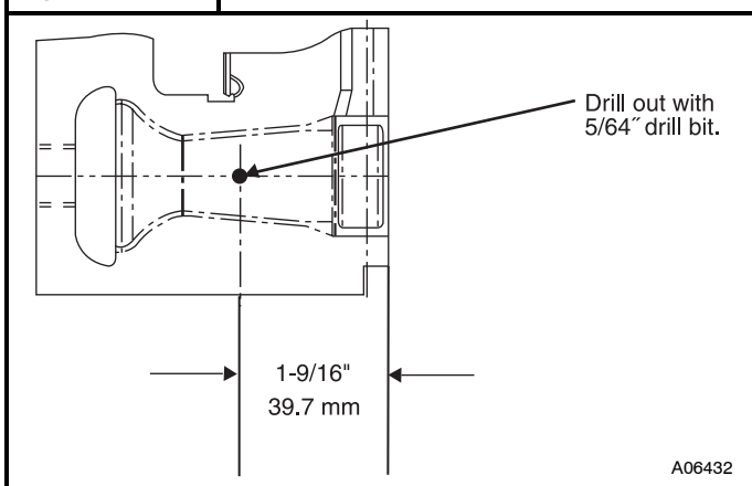
Figure 8 Mixer Screw Location
