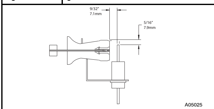
Figure 9 Igniter Position - Side View
