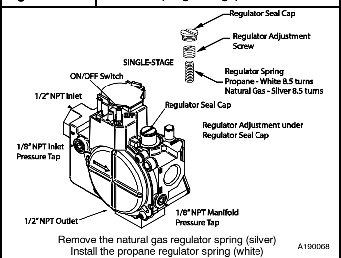
Figure 10 Gas Valve (Single Stage)
